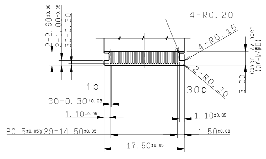
DETAIL A (S=2/1)
