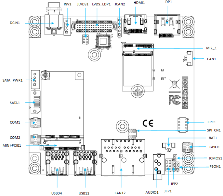
Figure 1.2 I/O Connectors
